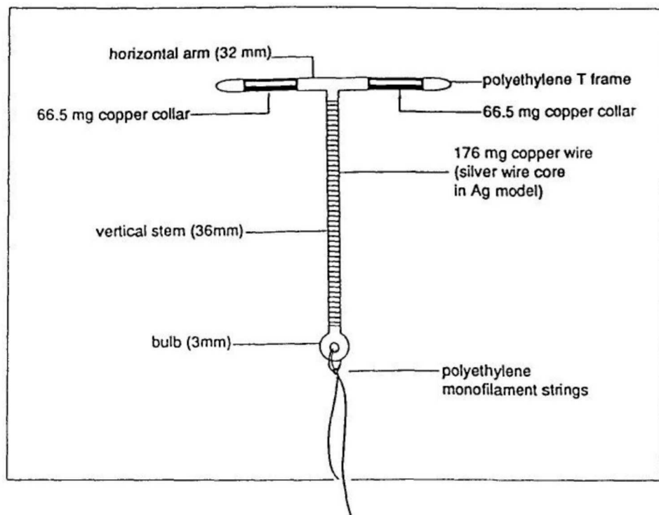
Figure 2: Copper T 380 IUD
